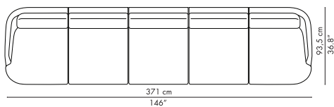
JH500 5-seater
