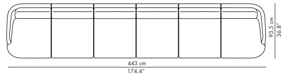
JH600 6-seater
