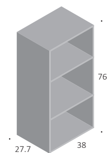
1/2 BOOKCASE MK74180
